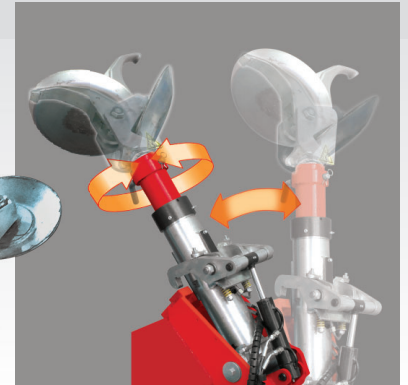
AUTOMATIC LIFTING and ROTATION
